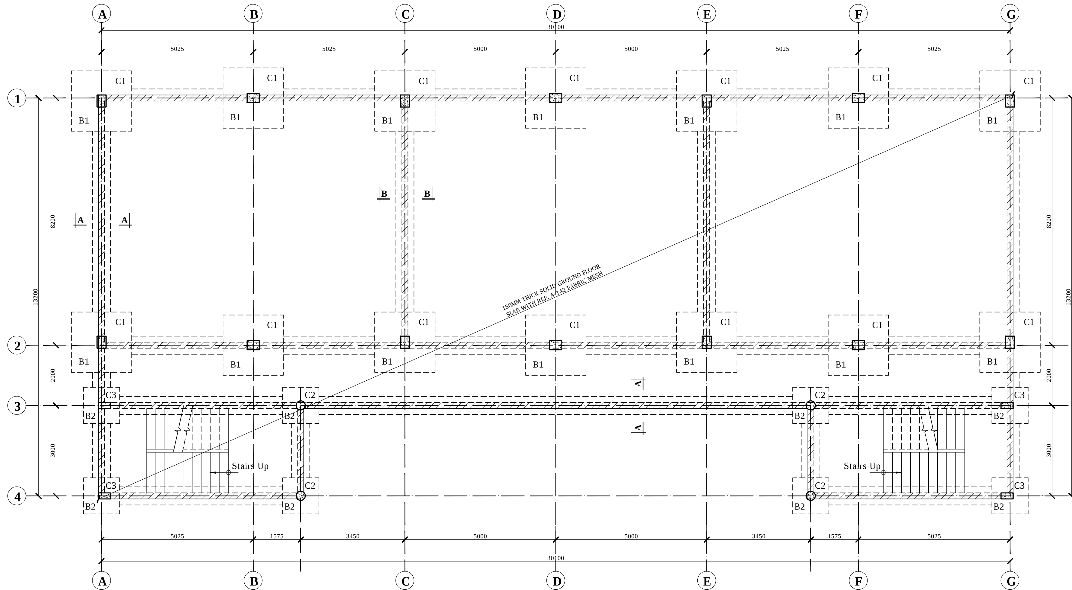
FOUNDATION/GROUND FLOOR LAYOUT
