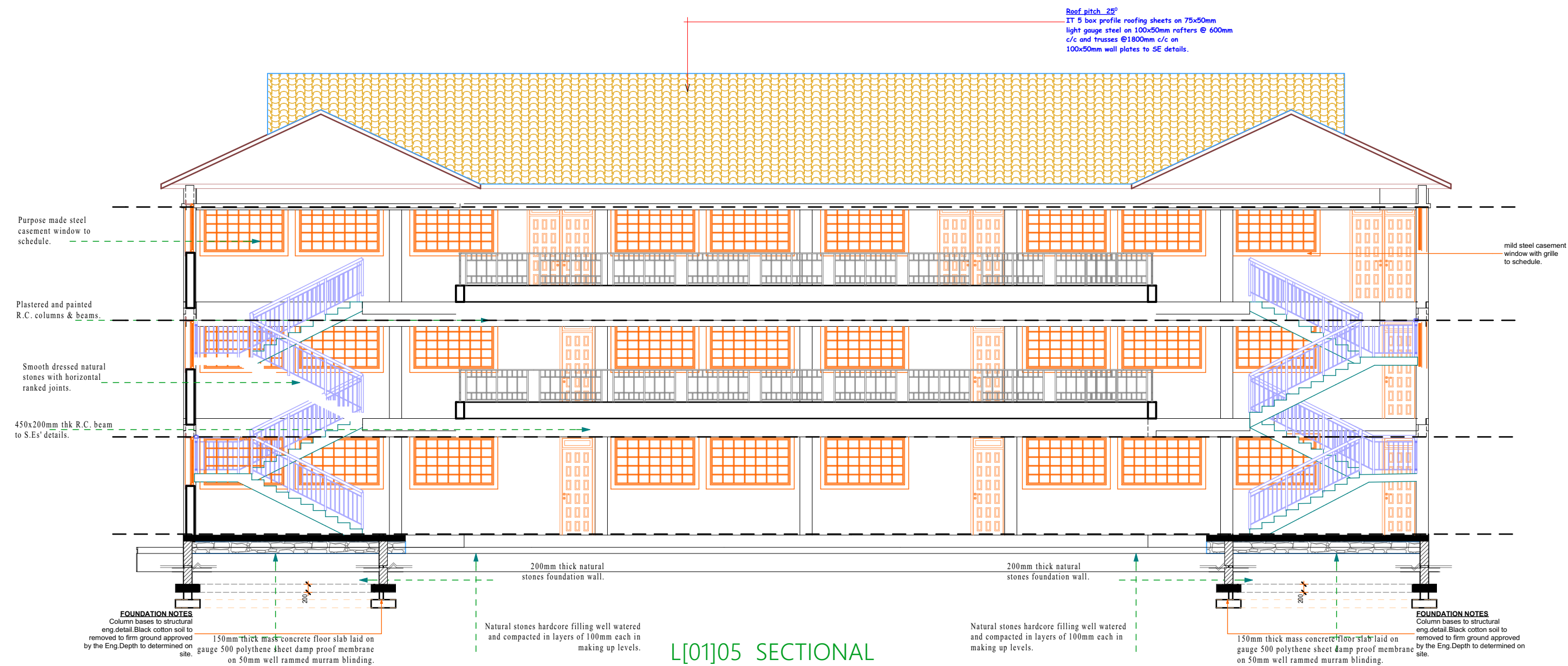
L[01]05 SECTIONAL ELEVATION (SCALE 1:75)
