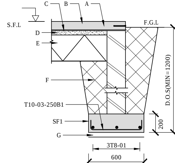
SEC C-C: EXTERNAL WALL STRIP FOOTING 'SF1'
