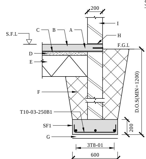
SEC A-A: EXTERNAL WALL STRIP FOOTING 'SF1'
