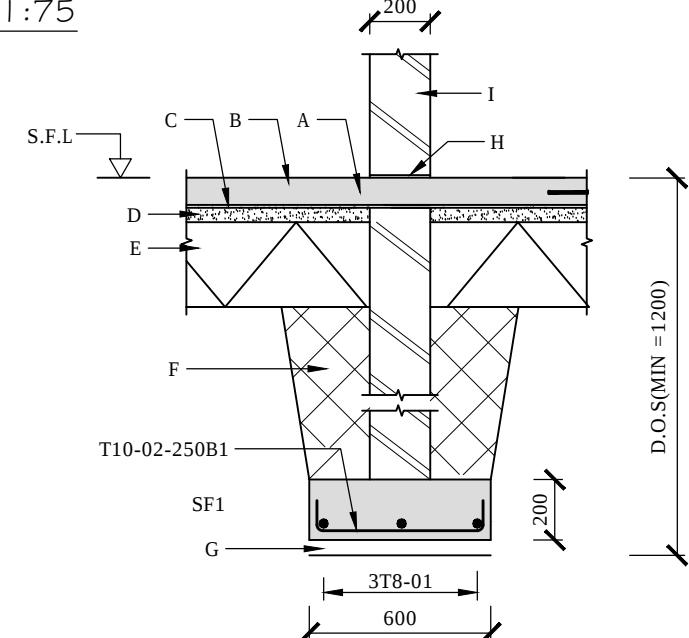
SEC B-B: INTERNAL WALL STRIP FOOTING 'SF1'
