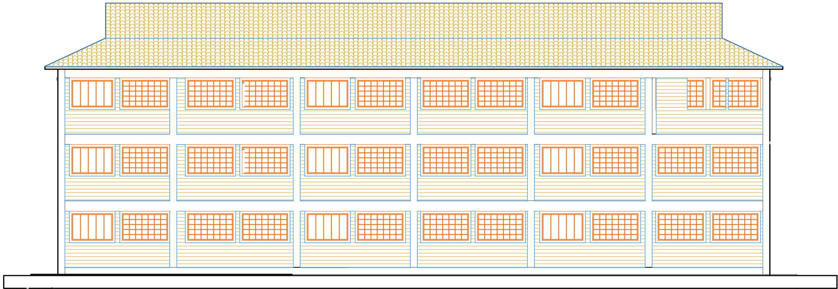
L[01]03 ELEVATION (SCALE 1:100)
