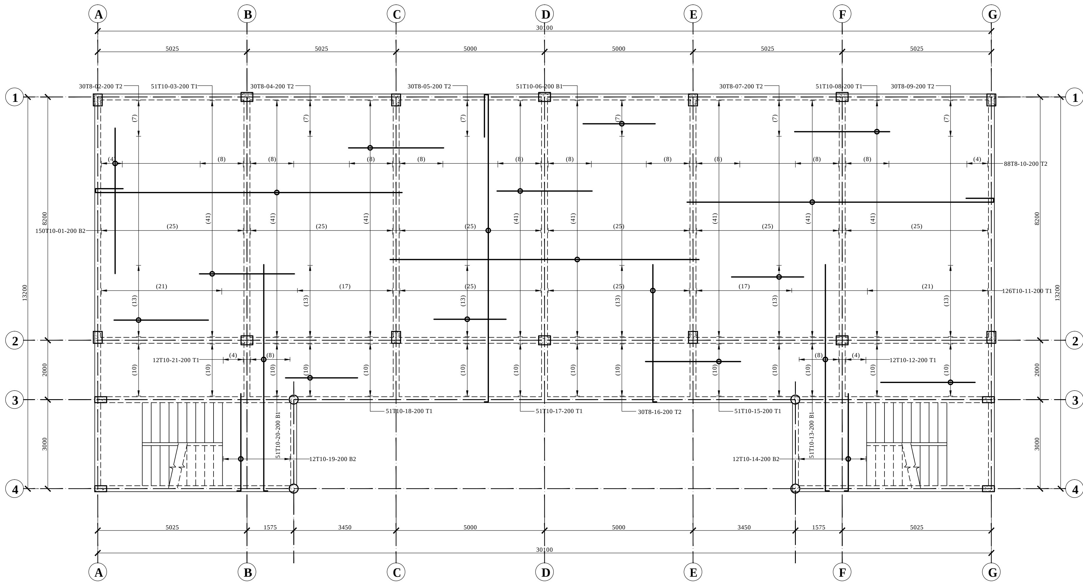
TYPICAL 1ST & 2ND FLOOR SLAB LAYOUT & R.C DETAILS Scale 1:75
