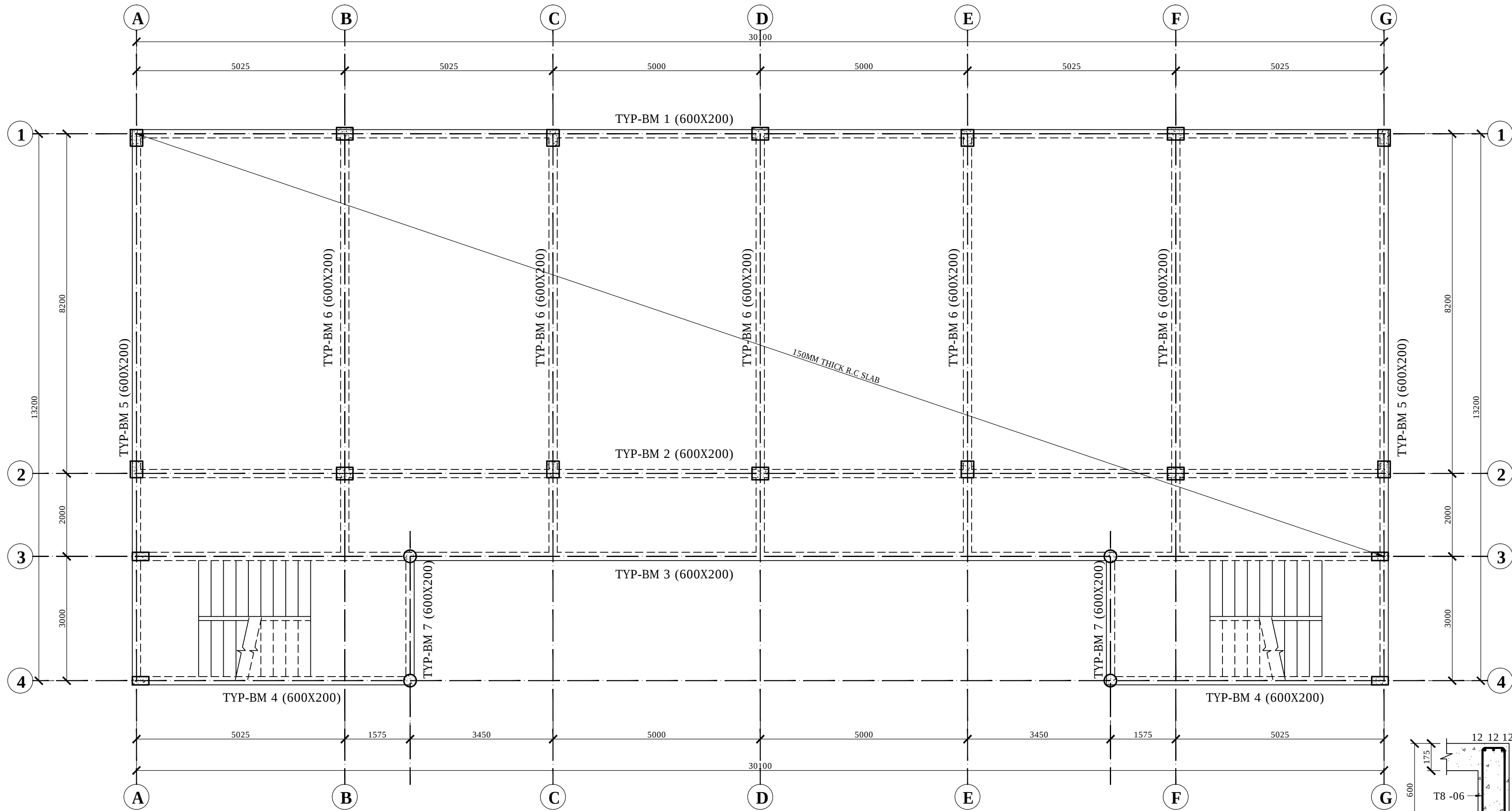
TYPICAL 1ST & 2ND FLOOR BEAM LAYOUT Scale 1:75
